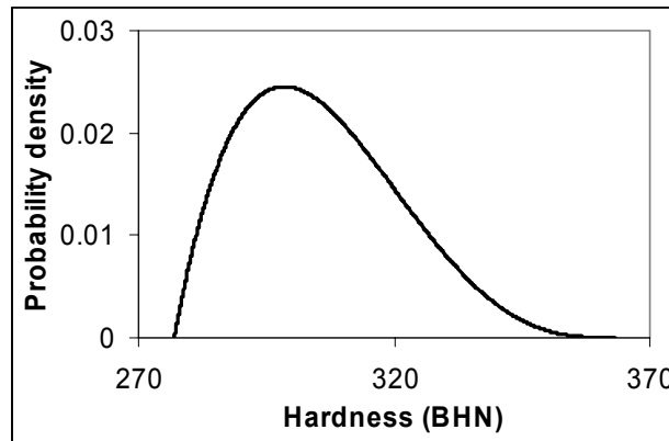
Figure 27. PDF of hardness distribution
